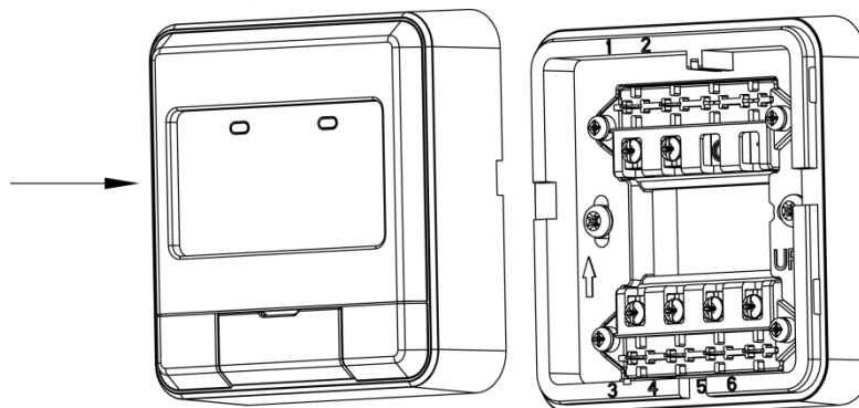
Figure 3-4 Installation (2)
