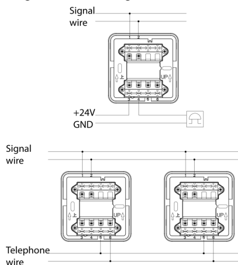
Figure 3-2 Mounting base (1)
