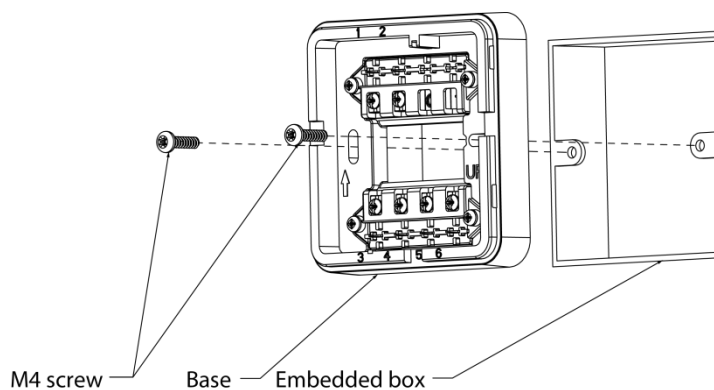
Figure 3-1 Installation (1)
