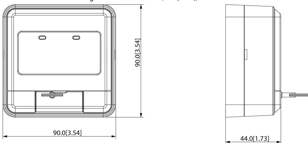
Figure 1-1 Dimensions (mm[inch])
