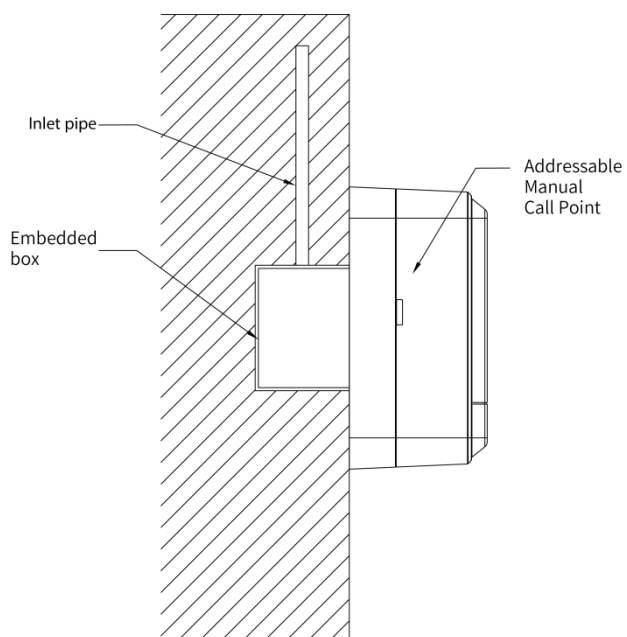
Figure 3-5 Installation (3)
