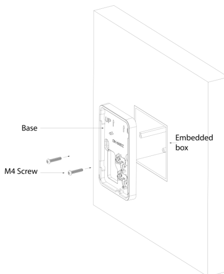
Figure 3-1 Installation (1)
