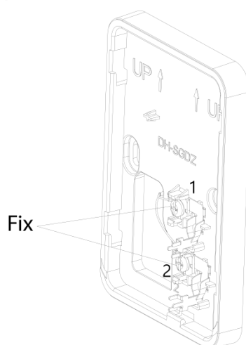
Figure 3-3 Installation (2)
