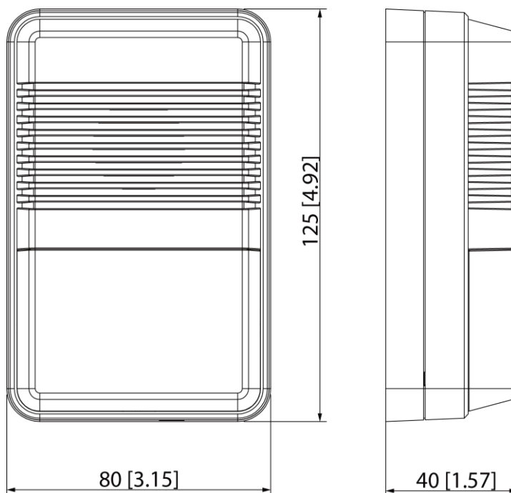
Figure 1-1 Dimensions (mm[inch])
