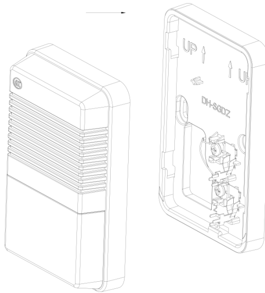
Figure 3-6 Installation (3)
