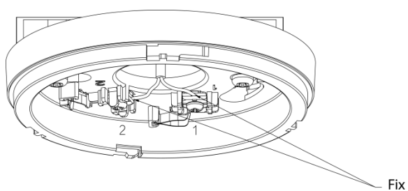
Figure 3-3 Installation (2)
