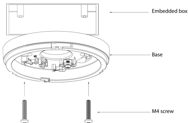
Figure 3-1 Installation (1)
